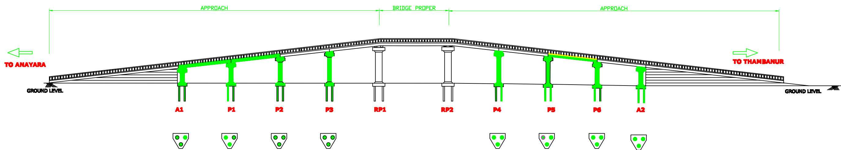
PILE FOUNDATION
